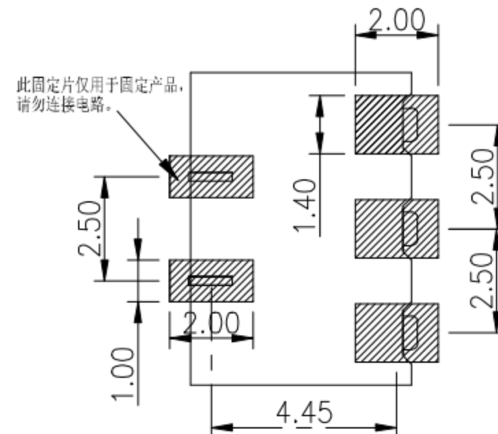
RECOMMENDED PCB LAYOUT TOP VIEW (.XX±0.05)
